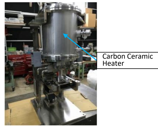
Sintering furnace
