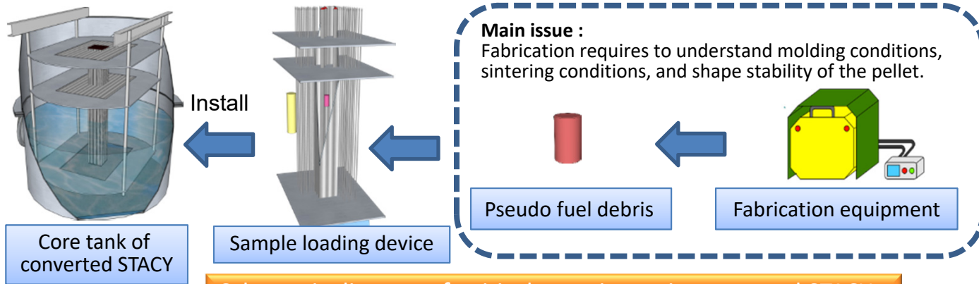
Schematic diagram of critical experiment in converted STACY
