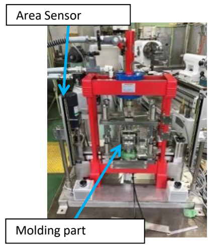
Molding machine
