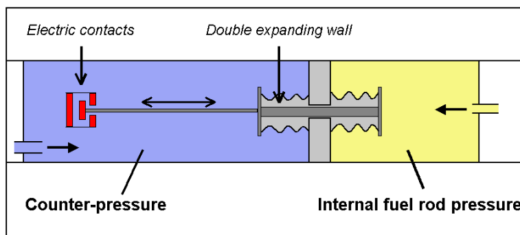
Fig. 4 Counter-pressure sensor principle
