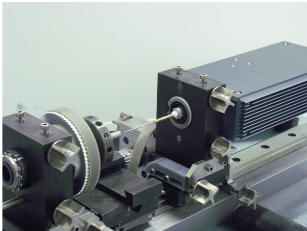
Fig. 1: Multi function machine tool during drill operation
