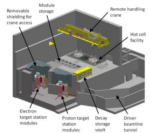
ARIEL: Advanced Rare IsotopE Laboratory – Next generation ISOL facility currently in design
