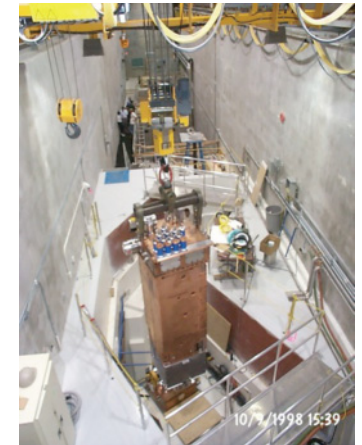
Target module transported with remote handling crane between target station and hot cell
