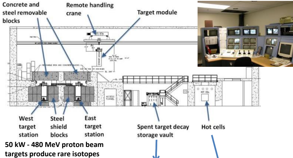
Target module transported with remote handling crane between target station and hot cell
